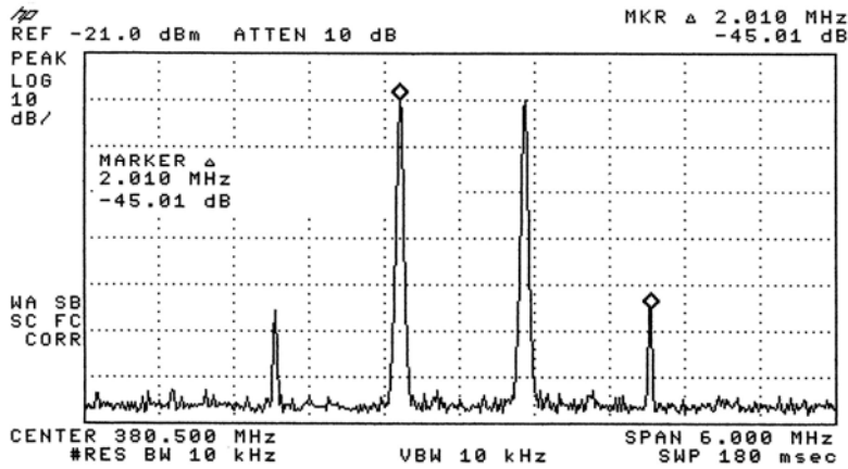
Two Tones 1 Watt Avg. Per Tone @ 380 & 381MHz IP3 = +52dBm
