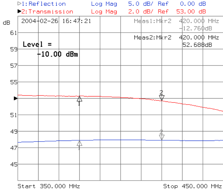
NP-512 Driving NP-513 Frequency Response Curve @ 20 Watts CW Output
