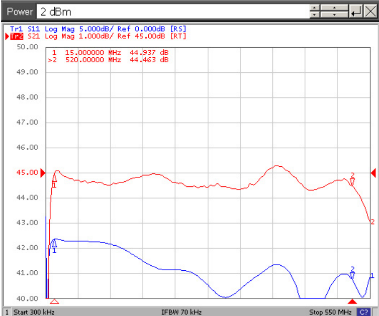
Frequency Response Curve @ 40 Watts Output
